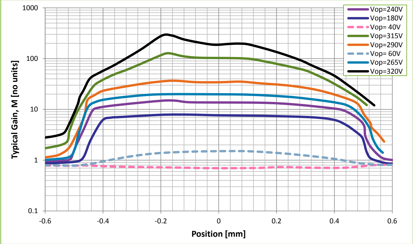
Figure 5 – Typical Gain as a function of Light Spot Position Test conditions: Case temperature = 22°C, Detector center = 0, Spot diameter= 0.0254 mm
