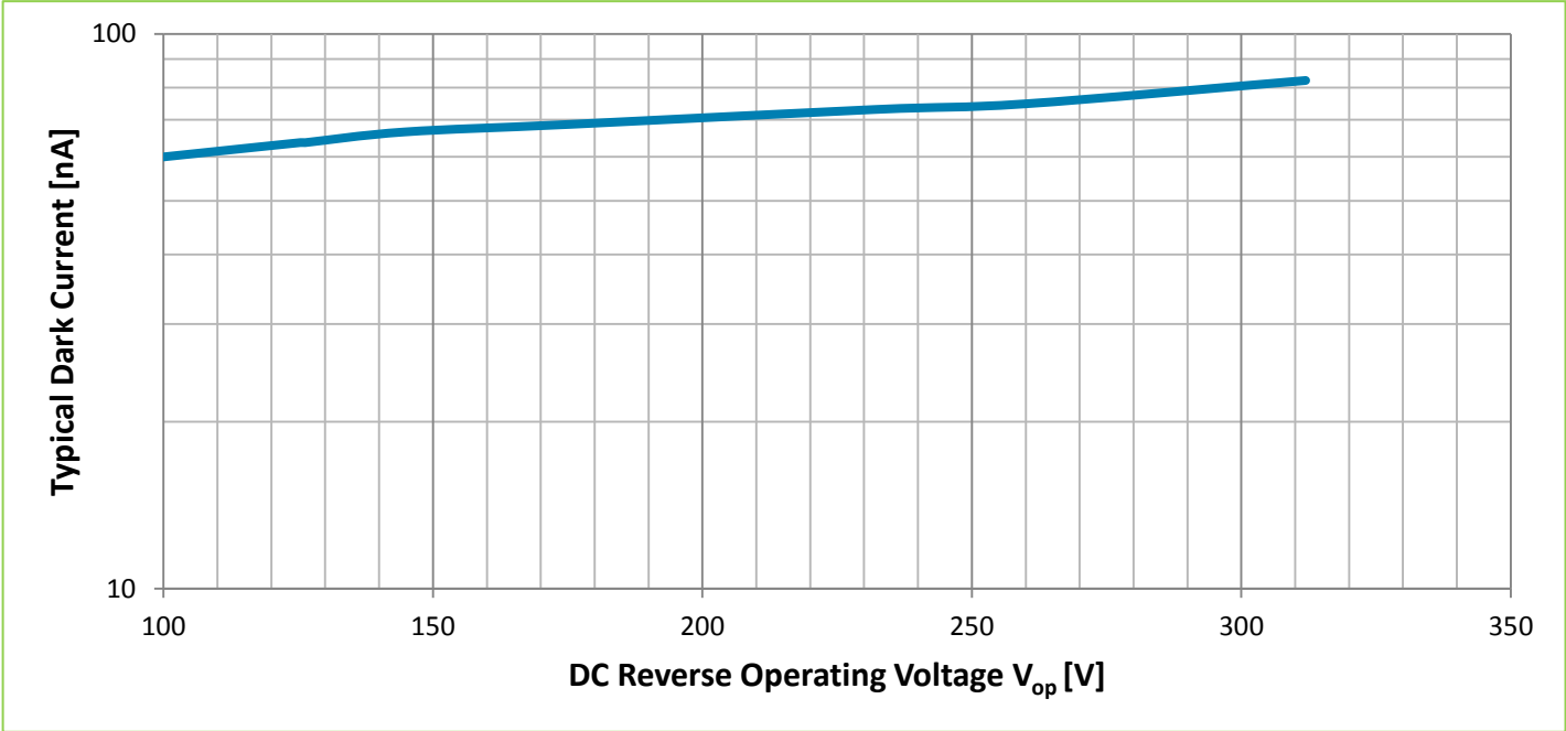
Figure 4 – Typical Dark Current as a function of Operating Voltage, V_{op} Test conditions: Case temperature = 22°C
