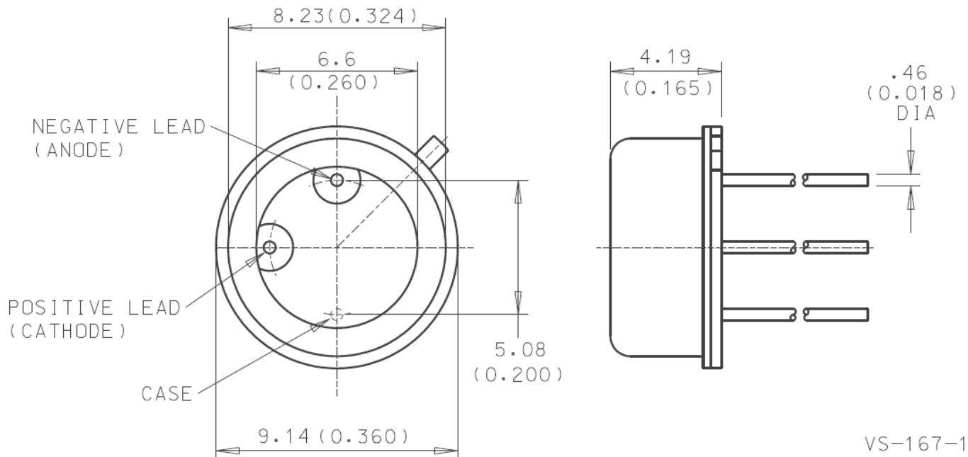
Figure 7 – Dimensional Outline
