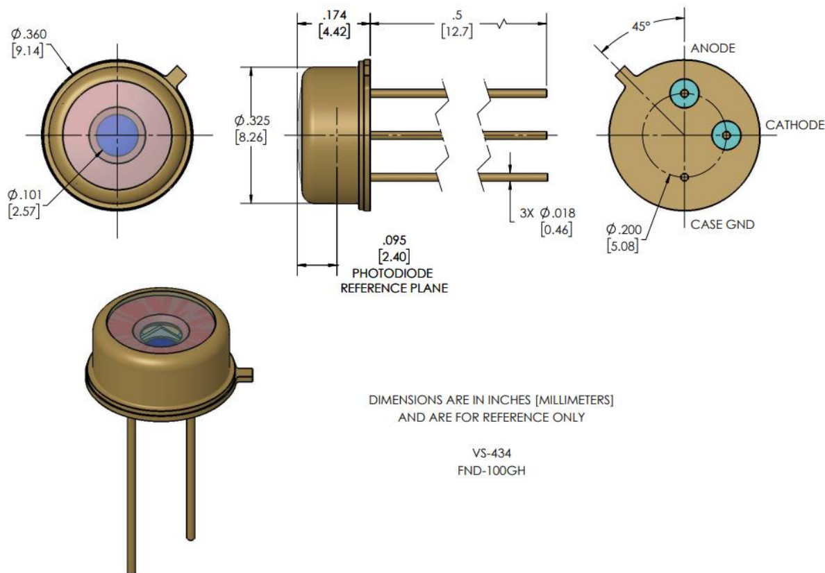
Figure 2: Dimensions
