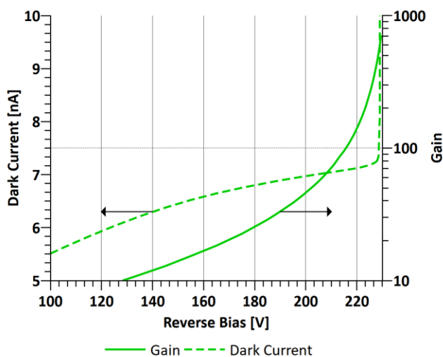
Figure 8: Typical Gain and Dark Current
