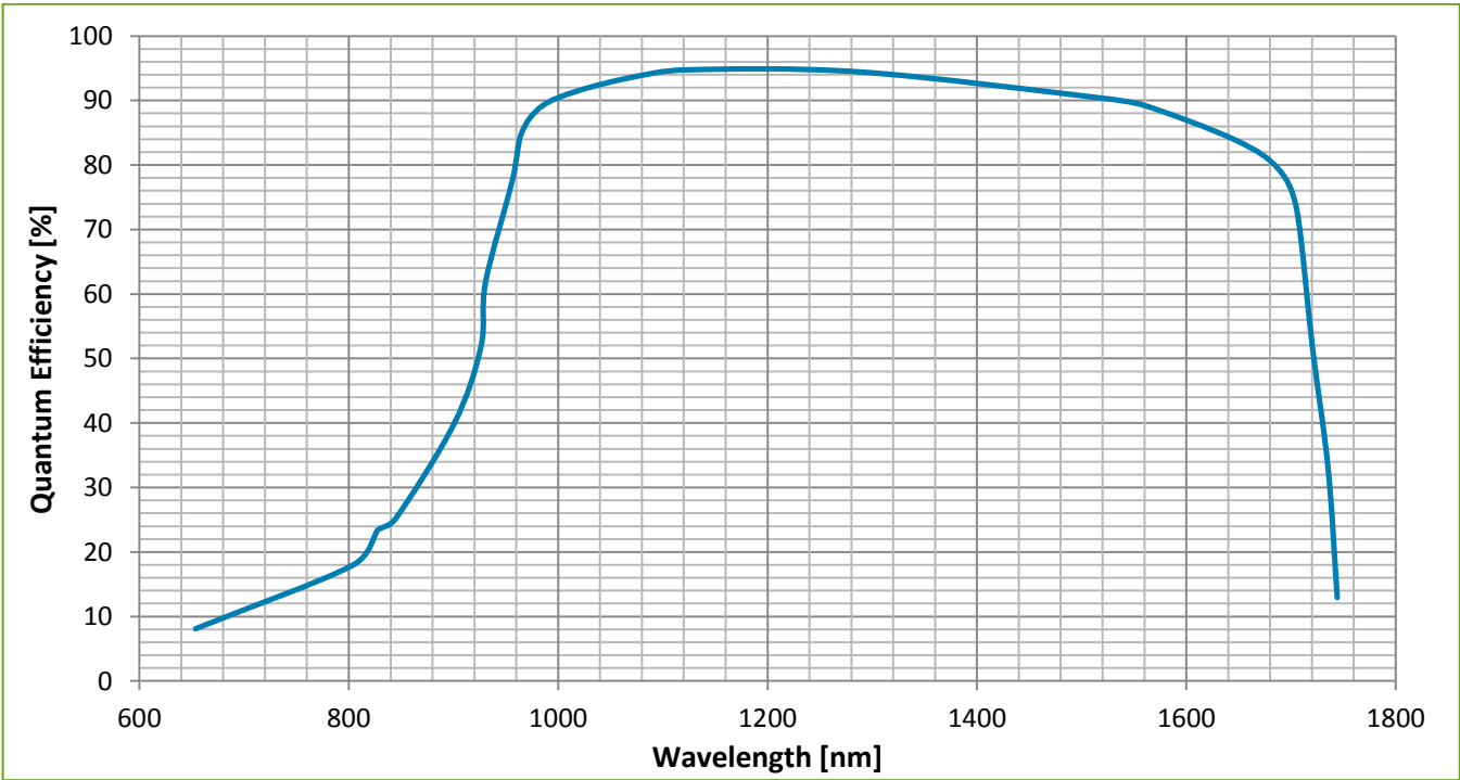
Figure 1 – Typical Quantum Efficiency as a function of Wavelength
