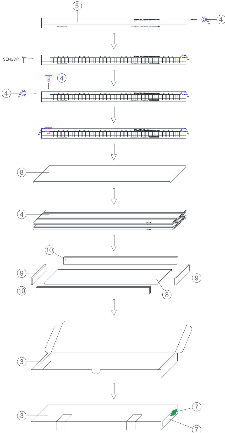
Figure 10: Information about the packaging of sensors.
