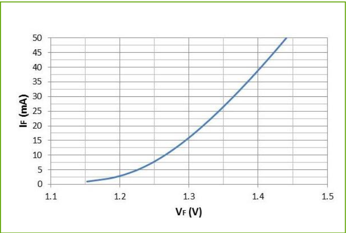
Figure 2: I-V Curve
