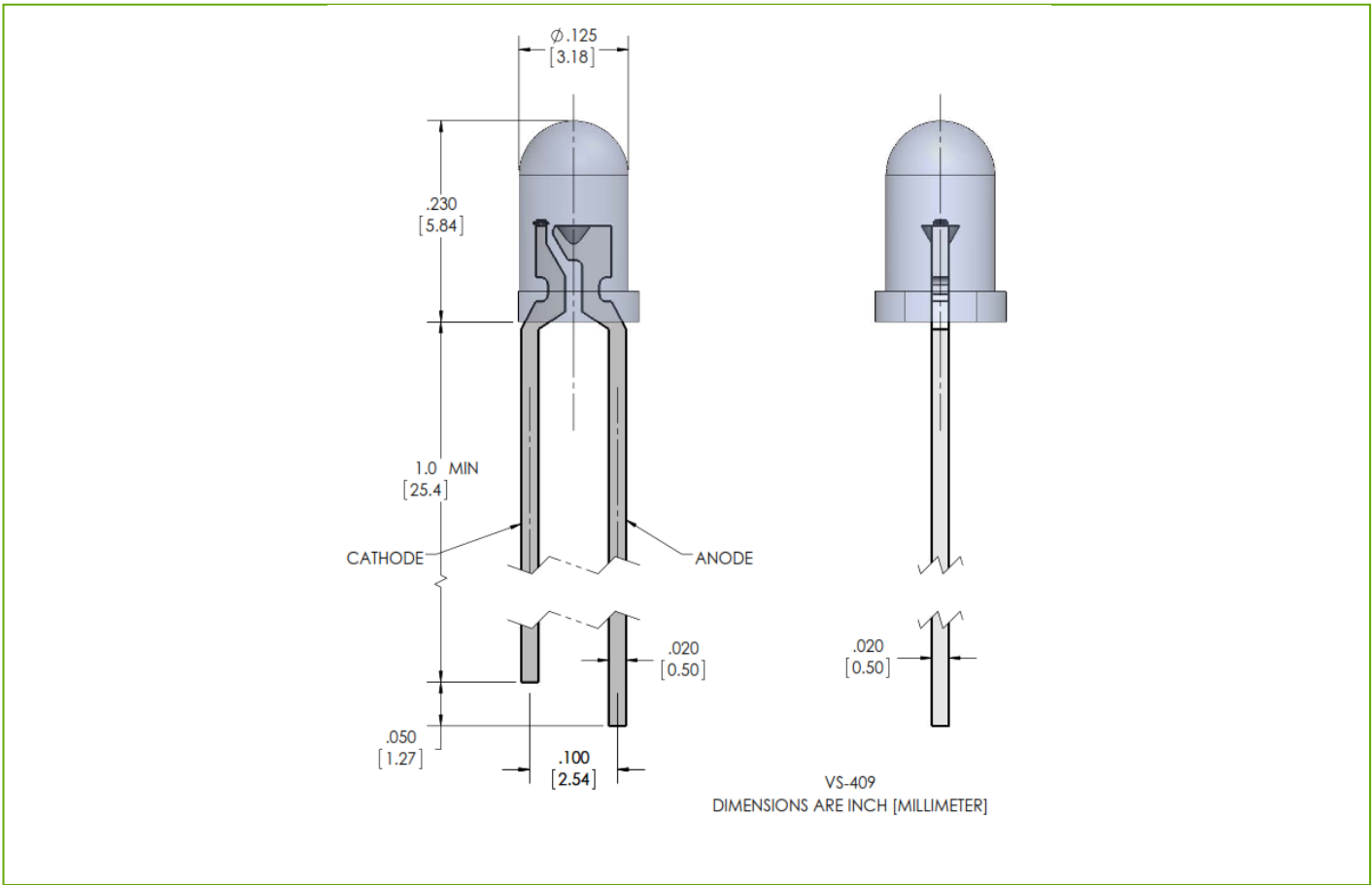
Figure 3: Mechanical Dimensions
