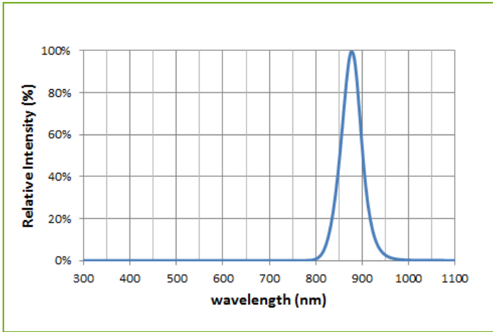
Figure 1: Emission Spectra
