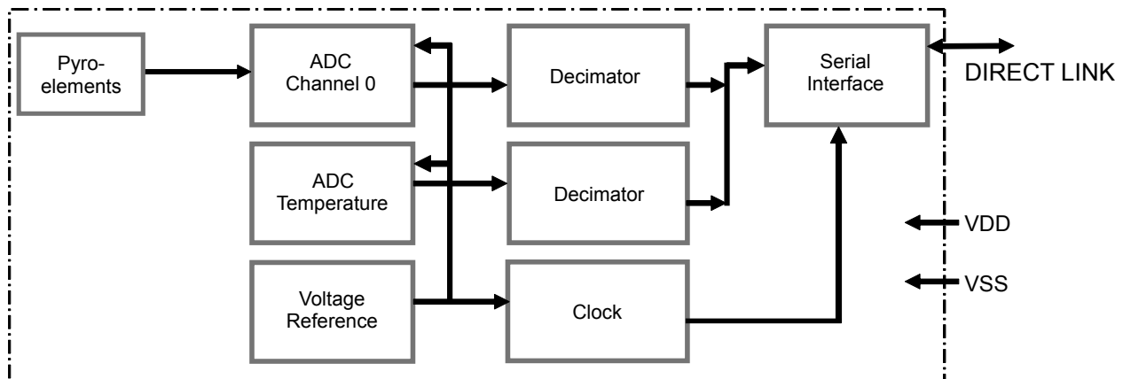
Figure 6: Block Diagram
