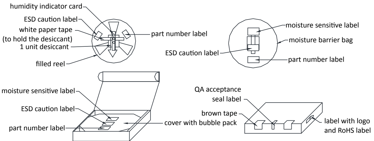
Figure 11: Packaging specifications
