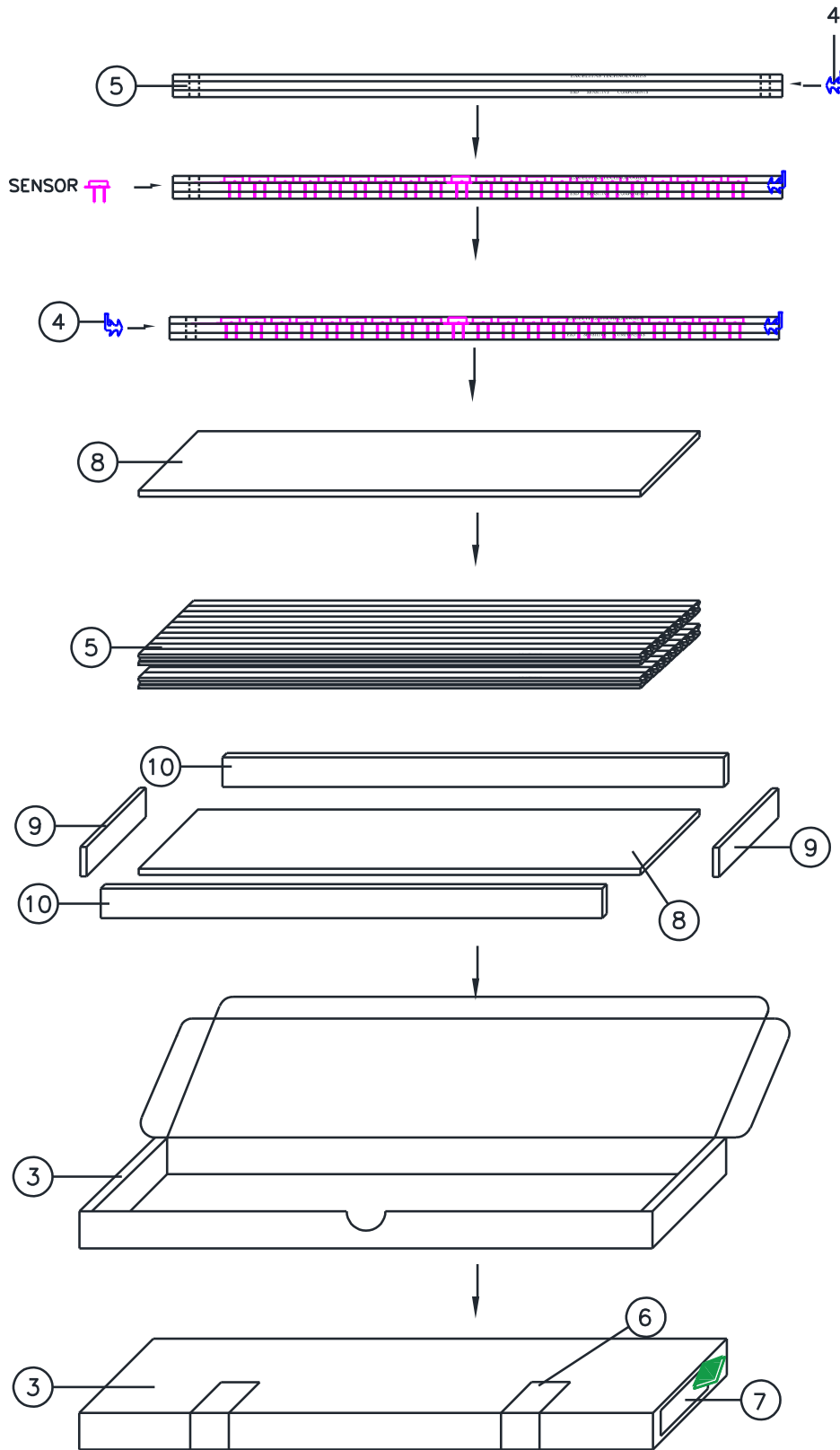
Figure 8: Information about the packaging of sensors.
