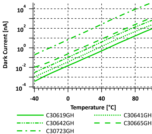
Figure 8: Typical Dark Current vs. Temperature
