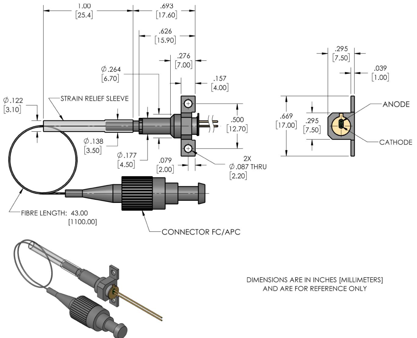
Figure 1: Mechanical Characteristics
