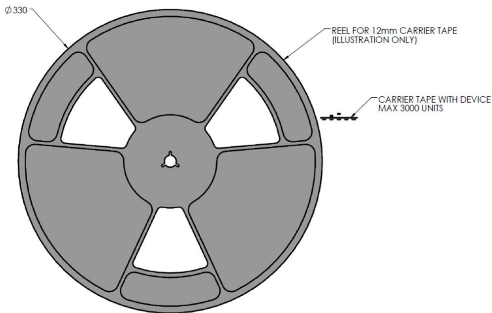
Figure 10: Tape and Reel Packaging Specification
