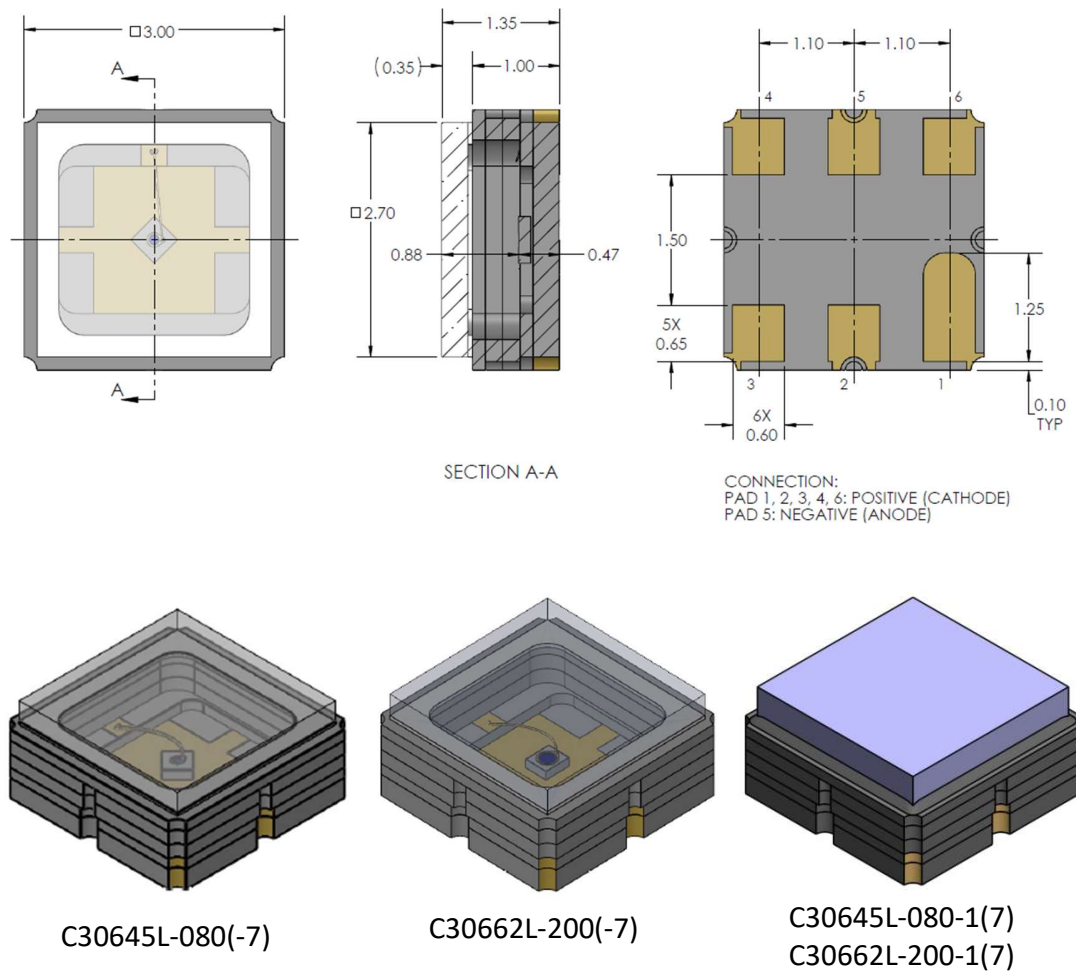
Figure 9: SMD Package Dimension C30645L-080 and C30662L-200
