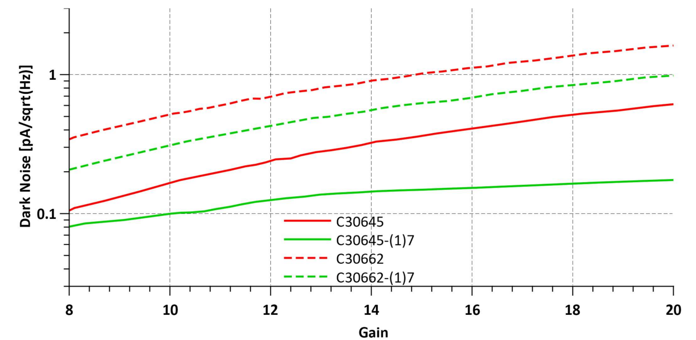
Figure 4: Typical Dark Noise vs. Gain
