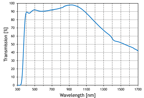
Transmission - inspec.x L 5.6/105 VIS/NIR 0.76x
