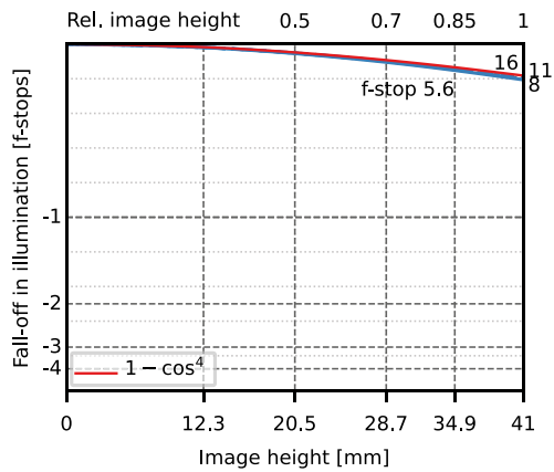
Fall-off in illumination
