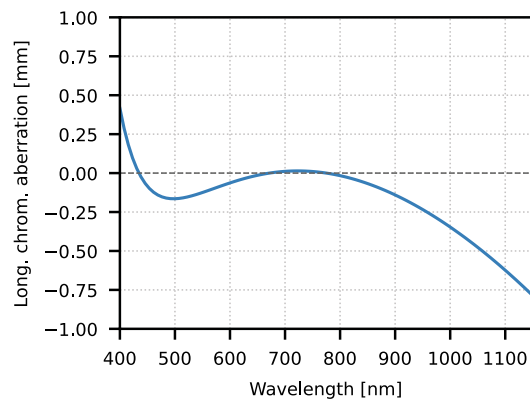
Long. chrom. aberration
