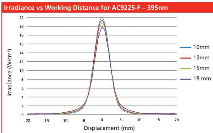
FIGURE 2: OmniCure AC9225-F with custom focusing lens for fiber curing applications.
