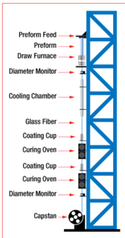
FIGURE 1: Schematic of a fiber optic drawing tower.
